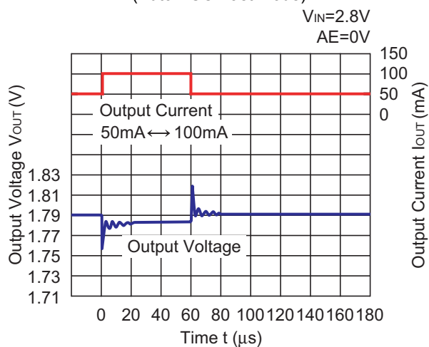
RP201x18xx (Auto ECO Fast Mode)
