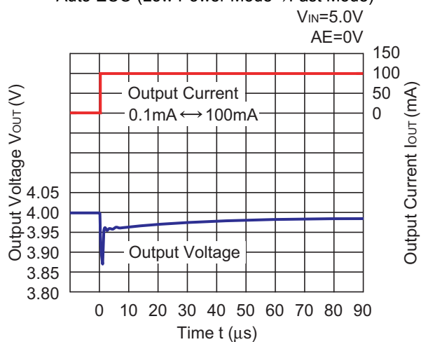
RP201x40xx Auto ECO (Low Power Mode→Fast Mode)
