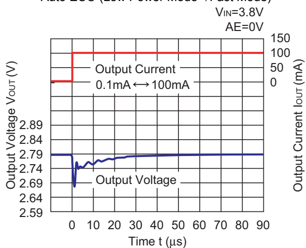
RP201x28xx Auto ECO (Low Power Mode→Fast Mode)
