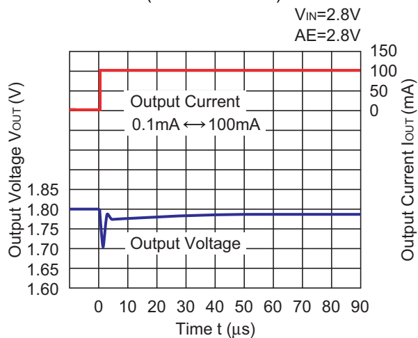
RP201x18xx (Fixed Fast Mode)
