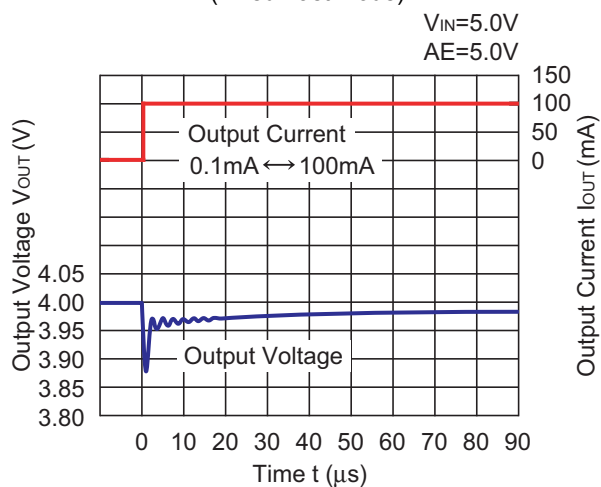
RP201x40xx (Fixed Fast Mode)
