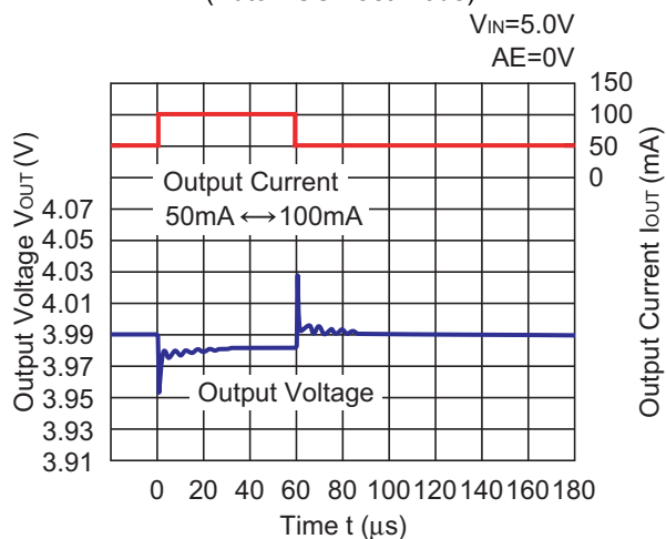
RP201x40xx (Auto ECO Fast Mode)
