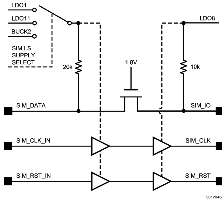
FIGURE 21. SIM Interface Level Shifters
