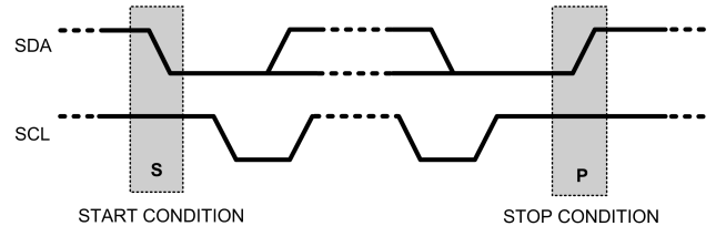
FIGURE 26. Start and Stop Conditions
