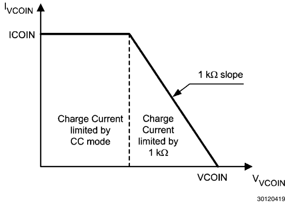
FIGURE 19. BBC IU Characteristics
