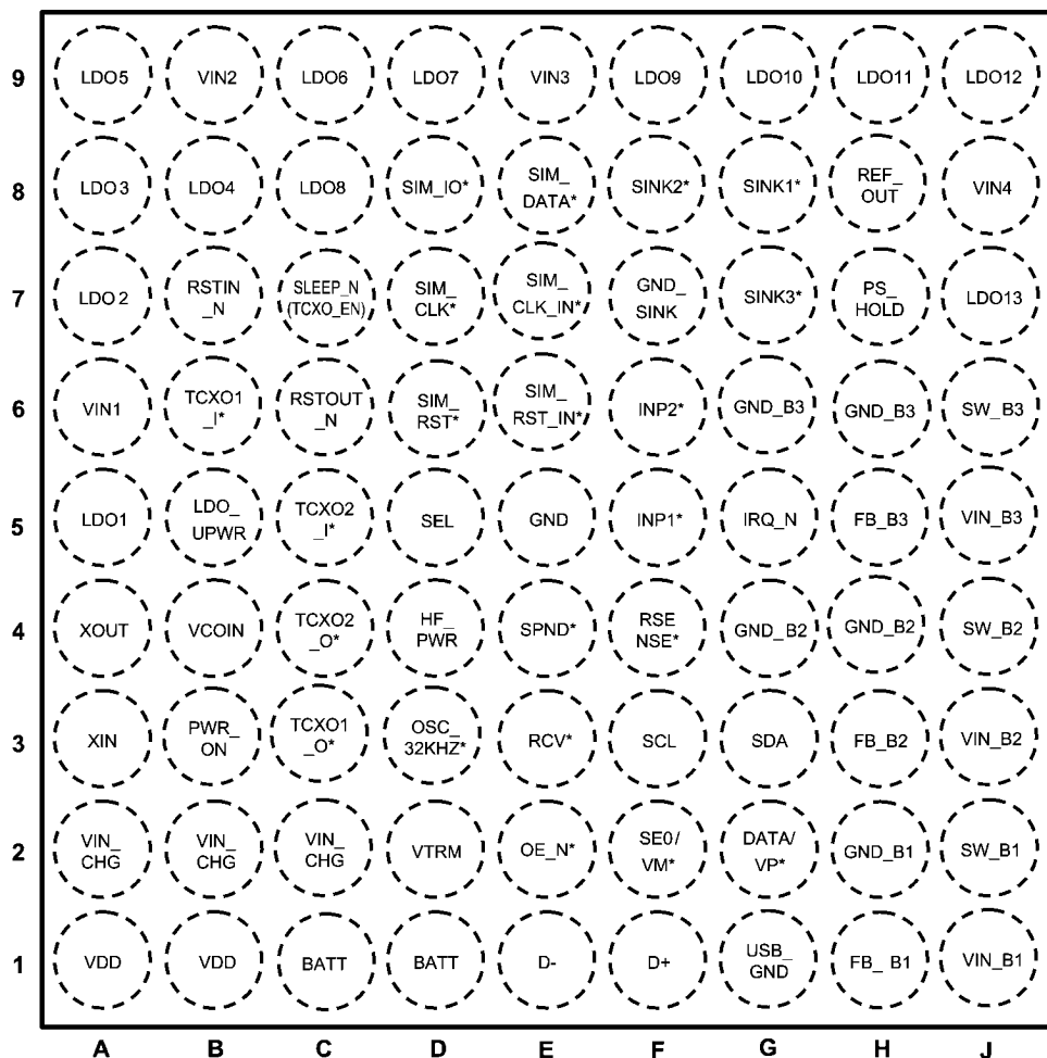
LP3925 (Top View)
