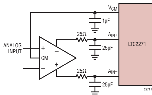
Figure 7. DC-Coupled Amplifier
