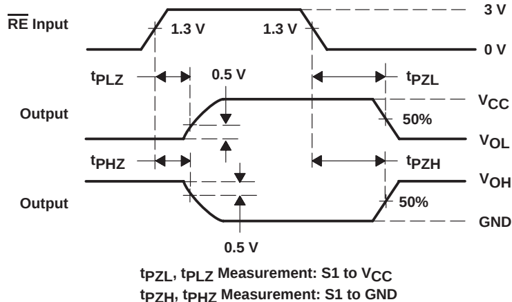
VOLTAGE WAVEFORMS
