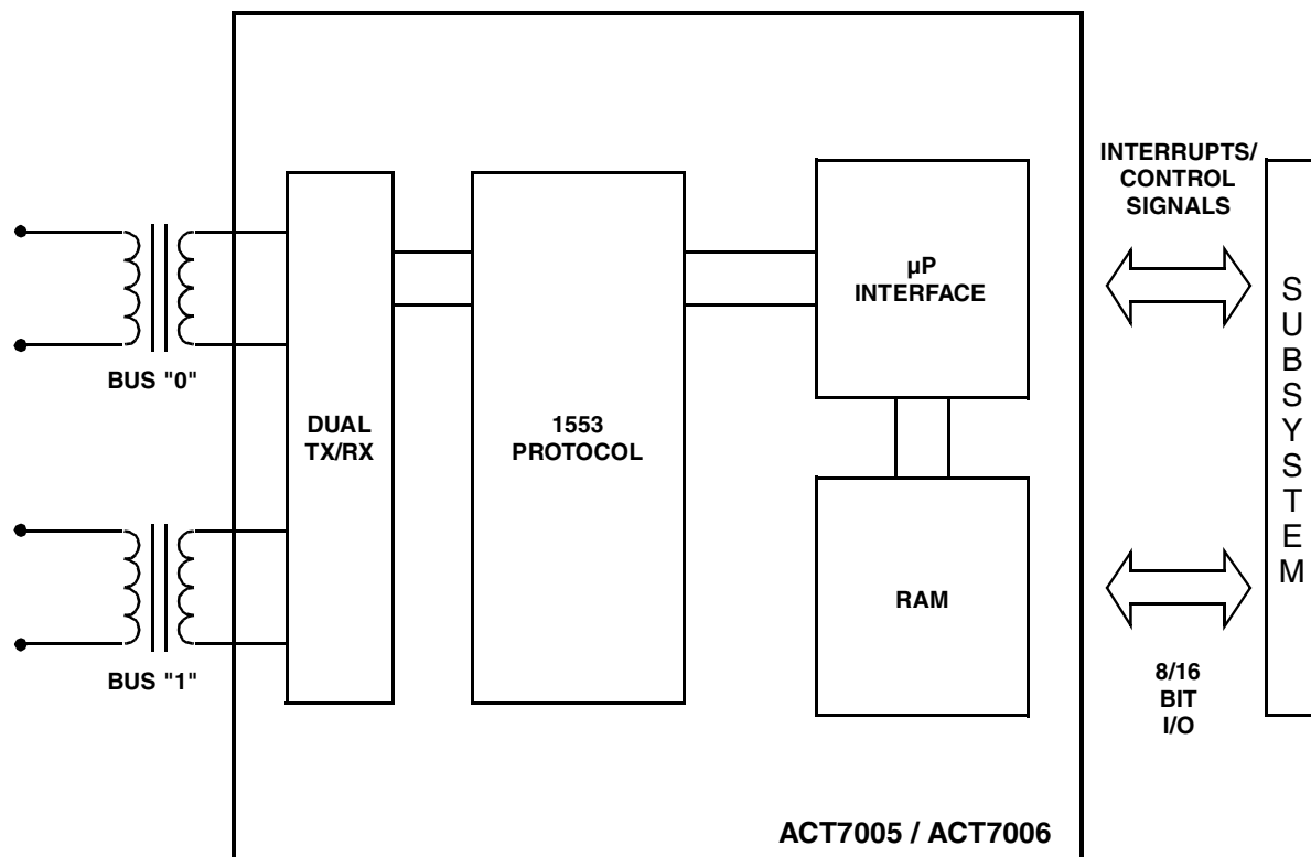
Block Diagram
