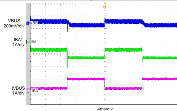
图 46. Load Transient During Supplement Mode
