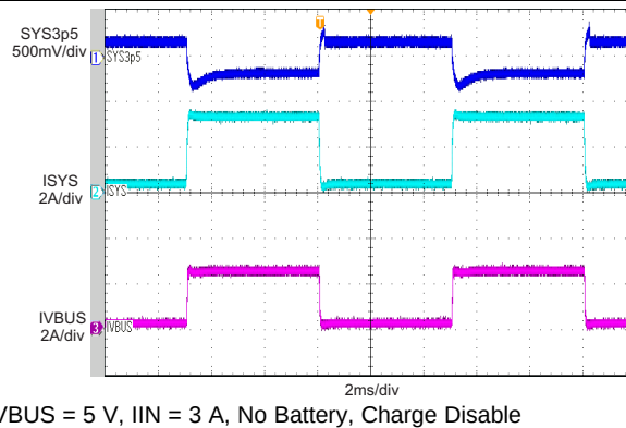
图 43. PWM Switching in Buck Mode
