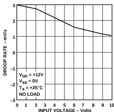
Figure 2. Droop Rate vs. Input Voltage
