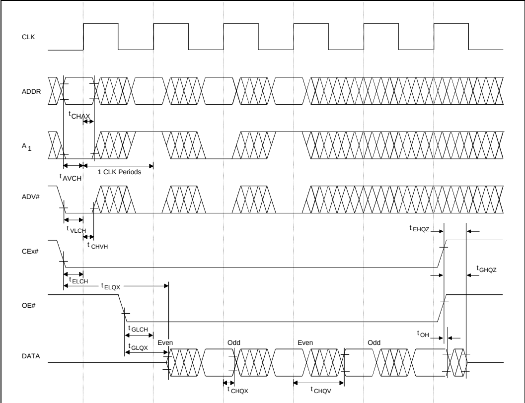
Figure 10. CLK Waveform
