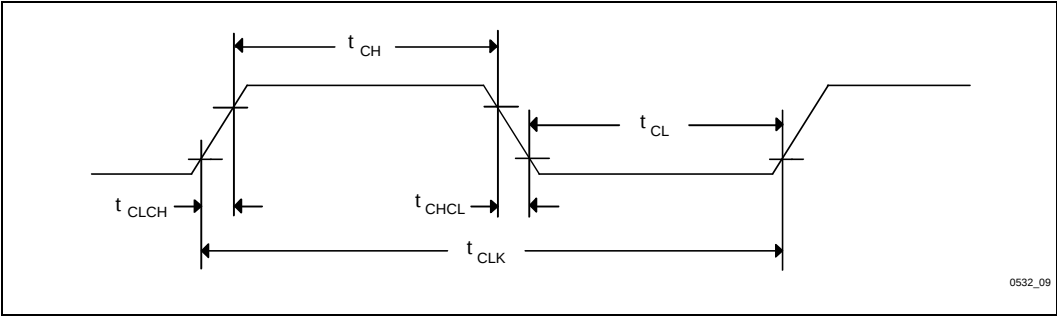
Figure 10. CLK Waveform
