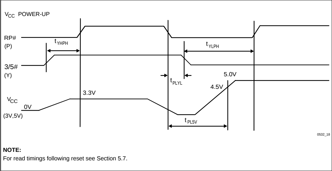
Figure 17. V CC Power-Up and RP# Reset Waveforms
