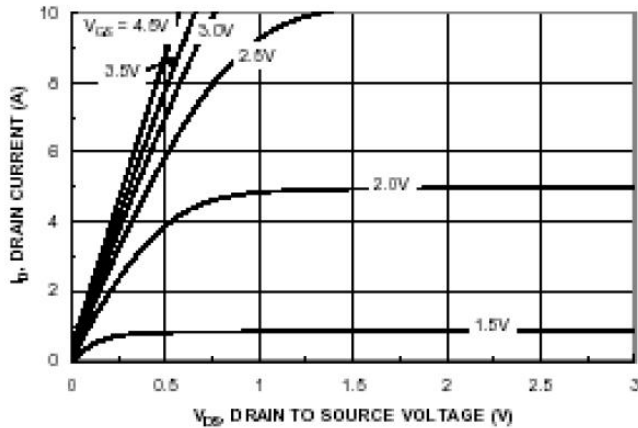
Figure 1. On-Region Characteristics.
