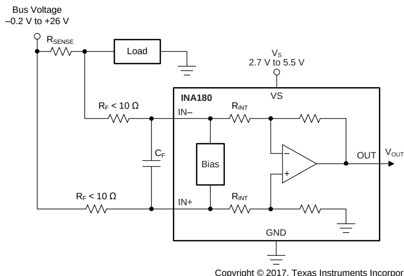
Figure 40. Filter at Input Pins
