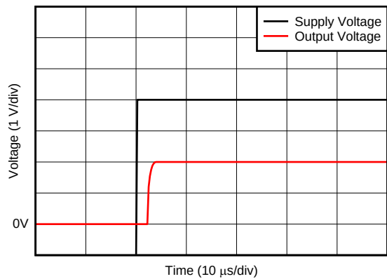
Figure 31. Start-Up Response
