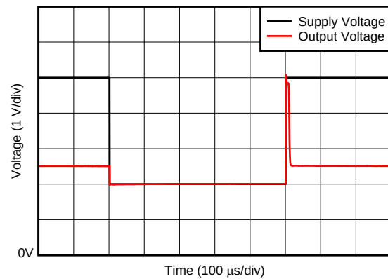
Figure 32. Brownout Recovery
