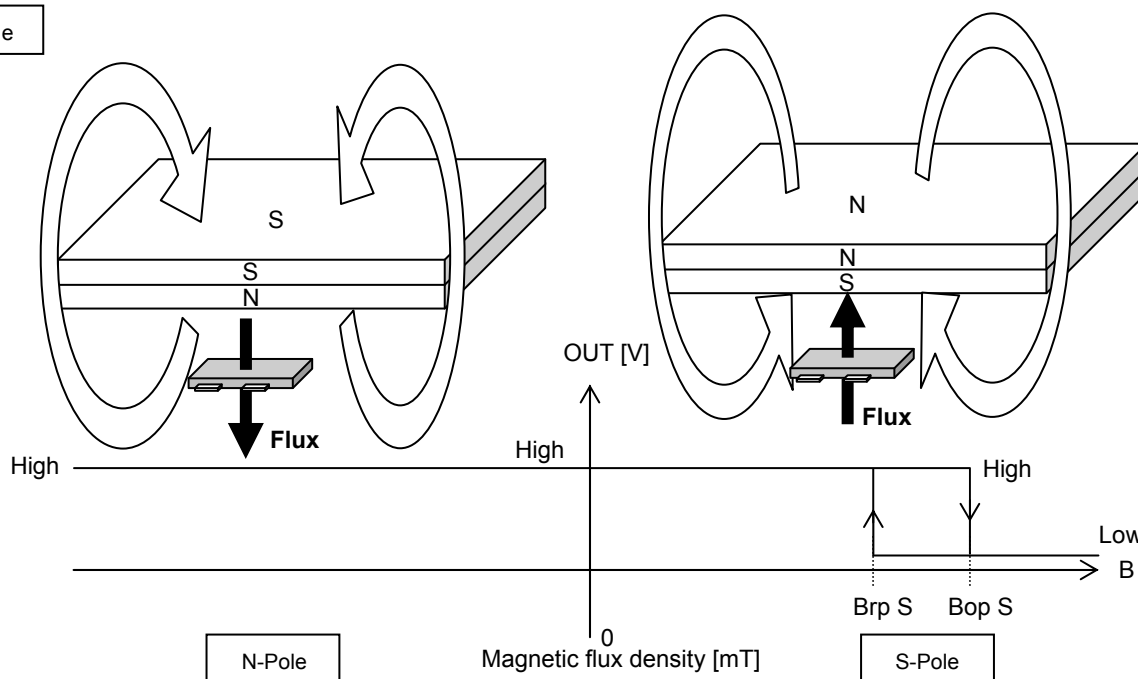
Fig.35 S-Pole Detection
