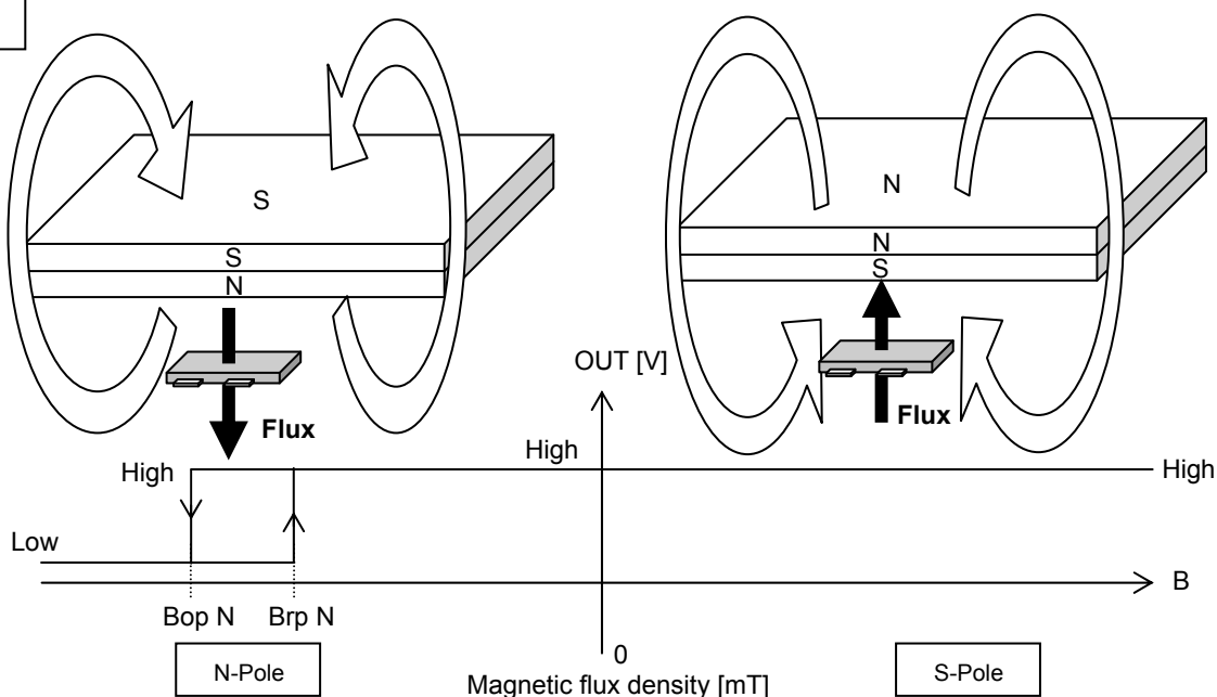
Fig.36 N-Pole Detection
