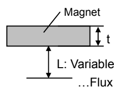
Fig.39 Magnet Dimensions and Flux Density Measuring Point
