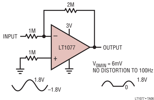
Half-Wave Rectifier
