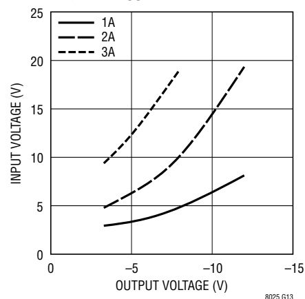
Minimum Input Voltage vs Negative V_{OUT}
