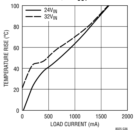
Junction Temperature Rise vs Load Current, 18V_{OUT}
