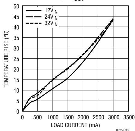
Junction Temperature Rise vs Load Current, 5V_{OUT}
