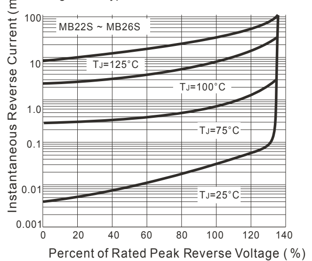
Fig. 4B - Typical Reverse Characteristics
