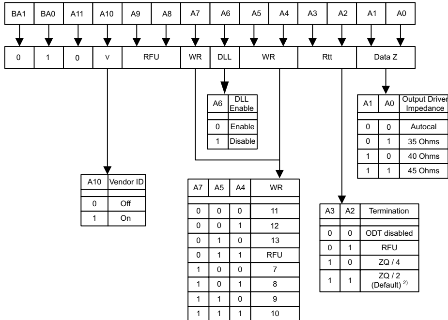
Extended Mode Register Bitmap for High-Speed Application
