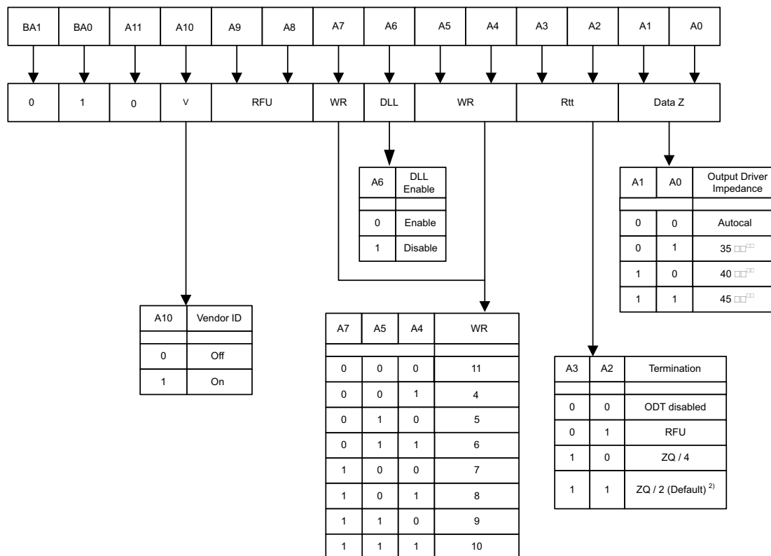
FIGURE 7 Extended Mode Register Bitmap for Mid-Range-Speed Application
