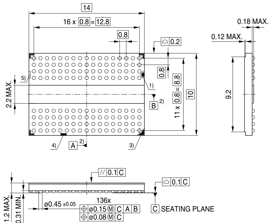
FIGURE 18 Package Outline PG-TFBGA-136-060
