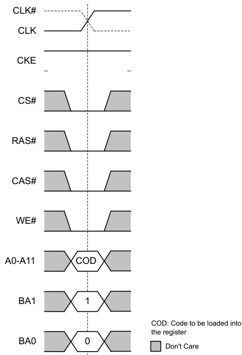
FIGURE 11 Extended Mode Register 2 Set Command
