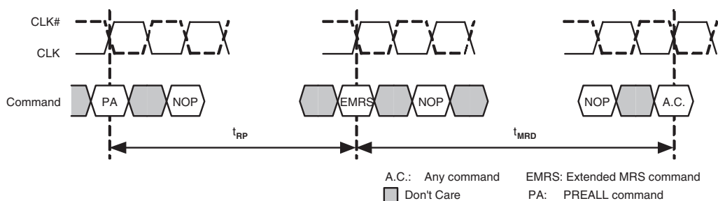
Extended Mode Register Set Timing
