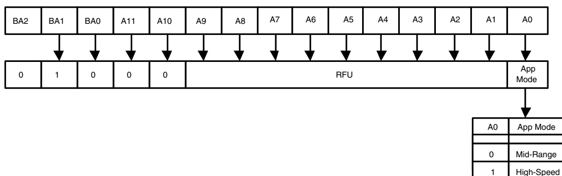
FIGURE 12 Extended Mode Register 2 Bitmap
