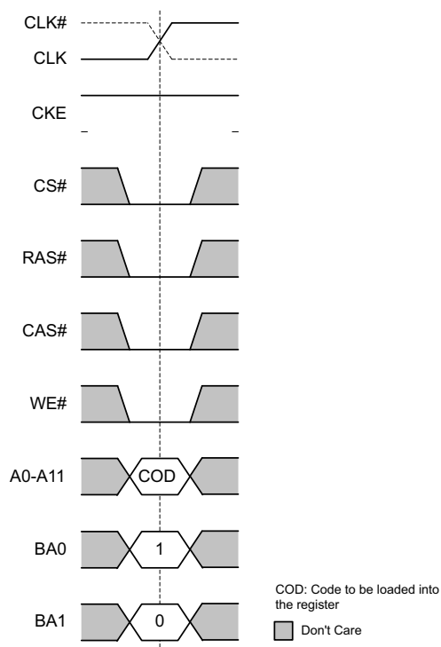
FIGURE 6 Extended Mode Register Set Command
