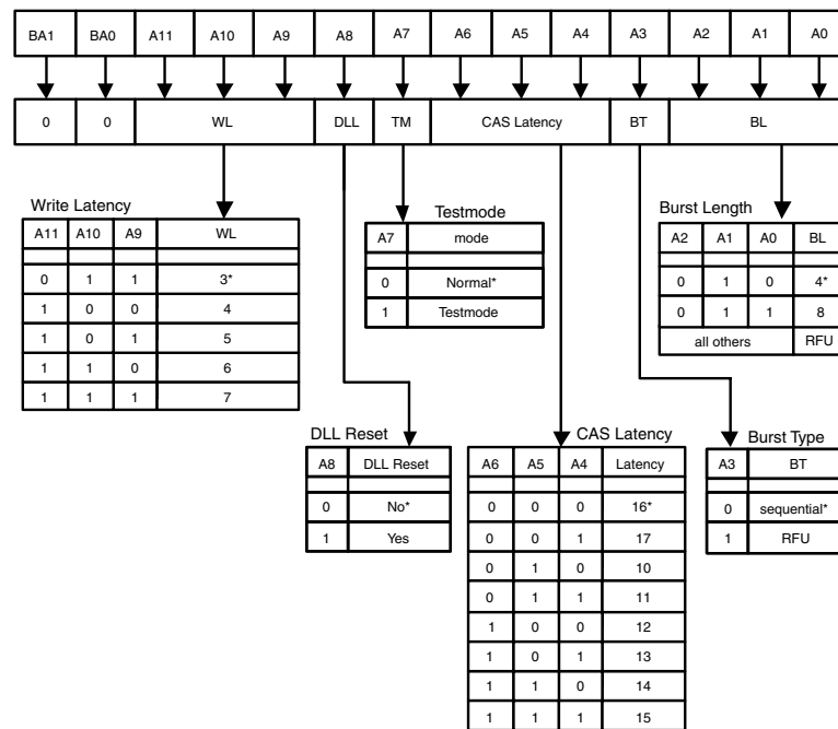
FIGURE 4 Mode Register Bitmap for High-Speed Application
