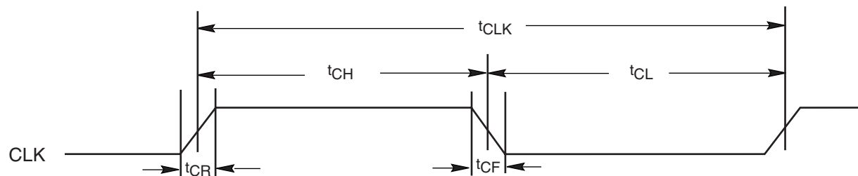
Figure 15. CLK Characterization
