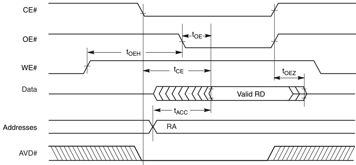
Figure 31. Asynchronous Mode Read with Latched Addresses
