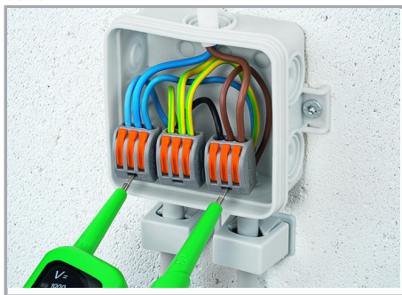
Testing via Profi-LED+ voltage tester (206-806).
