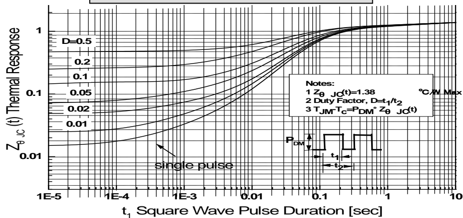
Transient Thermal Response Curve For JCS5N50VC/RC
