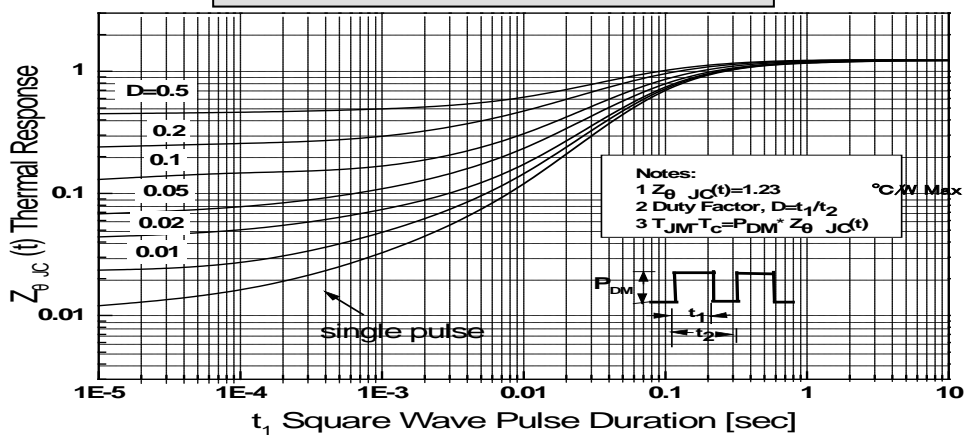
Transient Thermal Response Curve For JCS5N50CC
