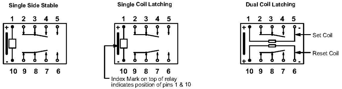
Pin Functions Bottom Views Shown
