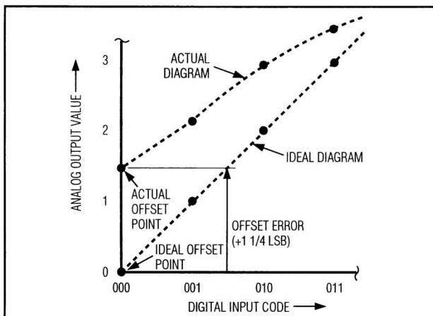
Figure 5c. Offset Error
