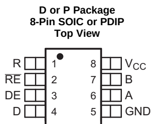
Pin Functions
