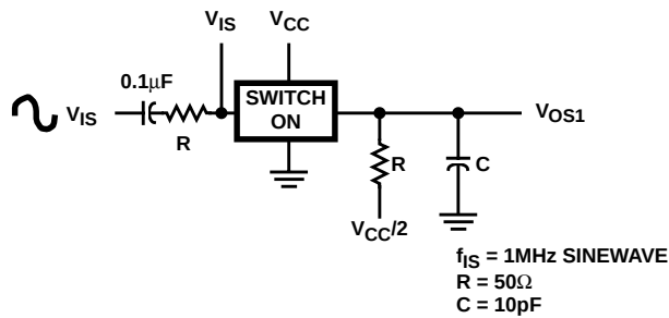
FIGURE 4. CROSTALK BETWEEN TWO SWITCHES TEST CIRCUIT
