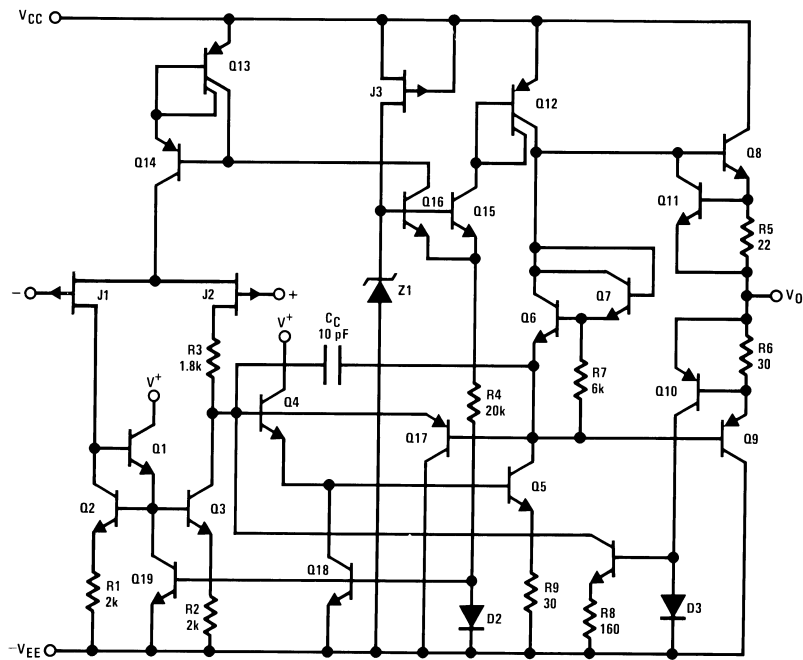
Figure 28. 1/2 Dual LF412-N-MIL
