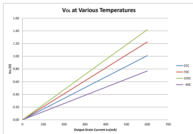
Figure 1. V_{OL} ( V_{DS} )
