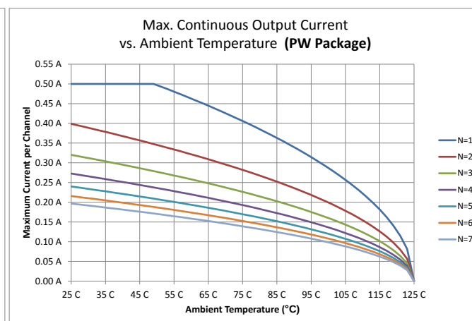
Figure 4. Maximum Output Current vs. Temperature (TSSOP)
