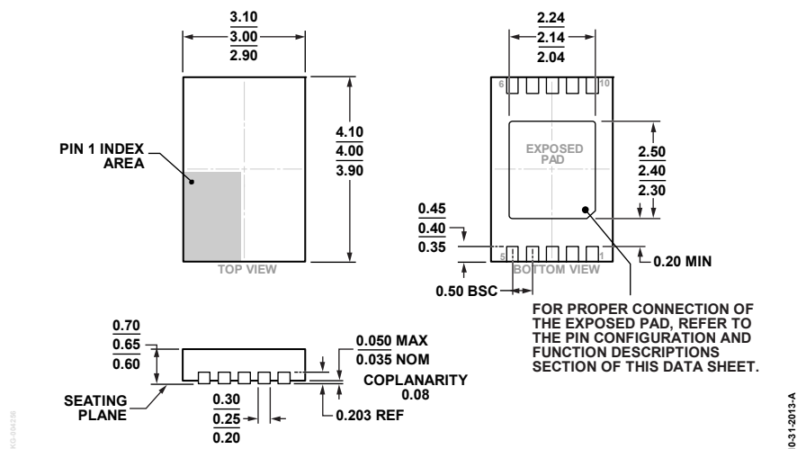
Figure 18. 10-Lead Lead Frame Chip Scale Package [LFCSP] 3 mm x 4 mm Body and 0.65 mm Package Height (CP-10-33) Dimensions shown in millimeters
