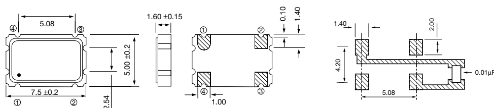
Figure 1) ECS-3951C/3953C Top, Side and Bottom views
