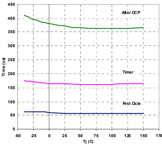
Figure 34. Start-up timer period vs. T_J
