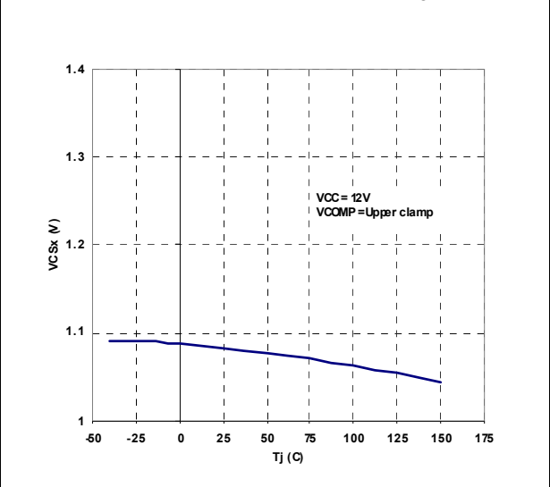
Figure 13. Vcs clamp vs. T_J
