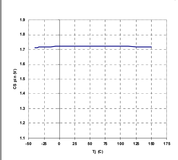
Figure 12. Inductor saturation threshold vs. T_J
