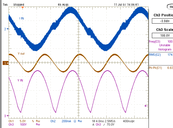
Figure 58. L6563H 100 W TM PFC evaluation board: input current waveform at 230-50 Hz - 100 W load
