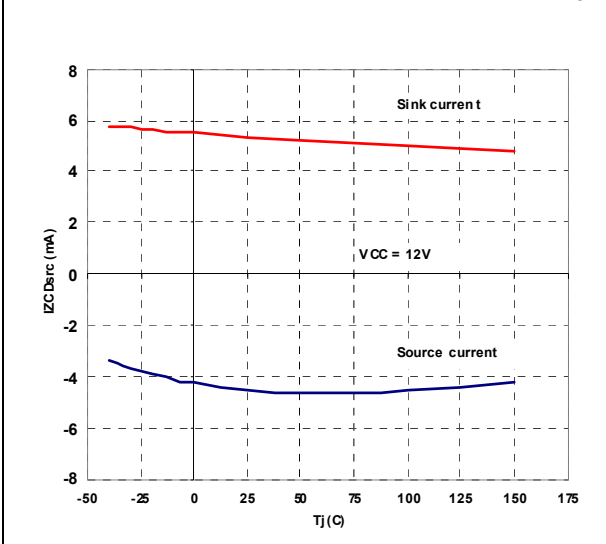
Figure 14. ZCD sink/source capability vs. T_J
