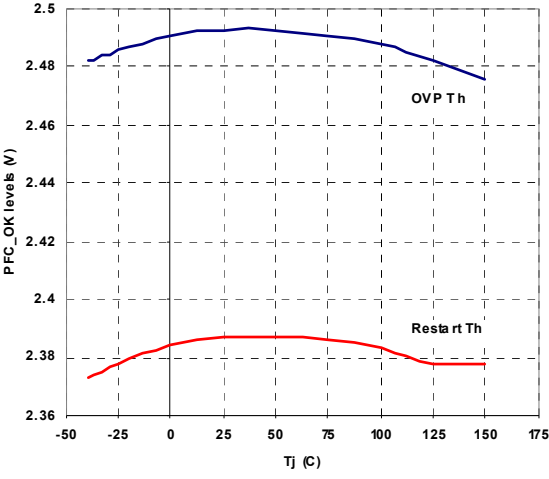
Figure 11. OVP levels vs. T_J
