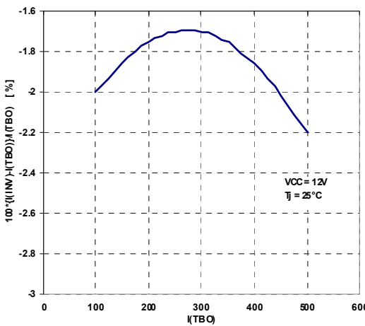
Figure 19. I_{INV} - I_{TBO} mismatch vs. I_{TBO} current
