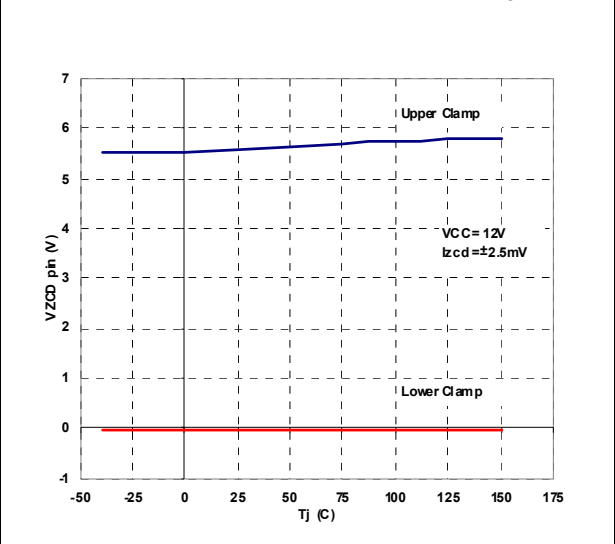
Figure 15. ZCD clamp level vs. T_J
