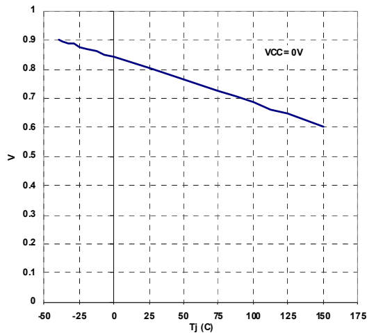
Figure 10. UVLO saturation vs. T_J
