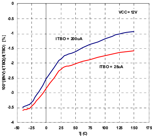
Figure 18. I_{INV} - I_{TBO} current mismatch vs. T_J
