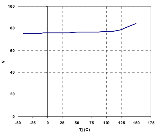
Figure 35. HV start voltage vs. T_J
