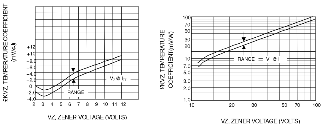
Fig. 2-TEMPERATURE COEFFICIENTS (-55 ^\circ C TO +150 ^\circ C TEMPERATURE RANGE; 90% OF THE UNITS ARE IN THE RANGES INDICATED.)
