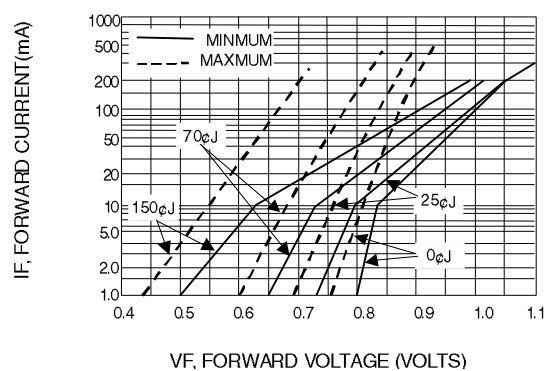
Fig. 10-TYPICAL FORWARD CHARACTERISTICS
