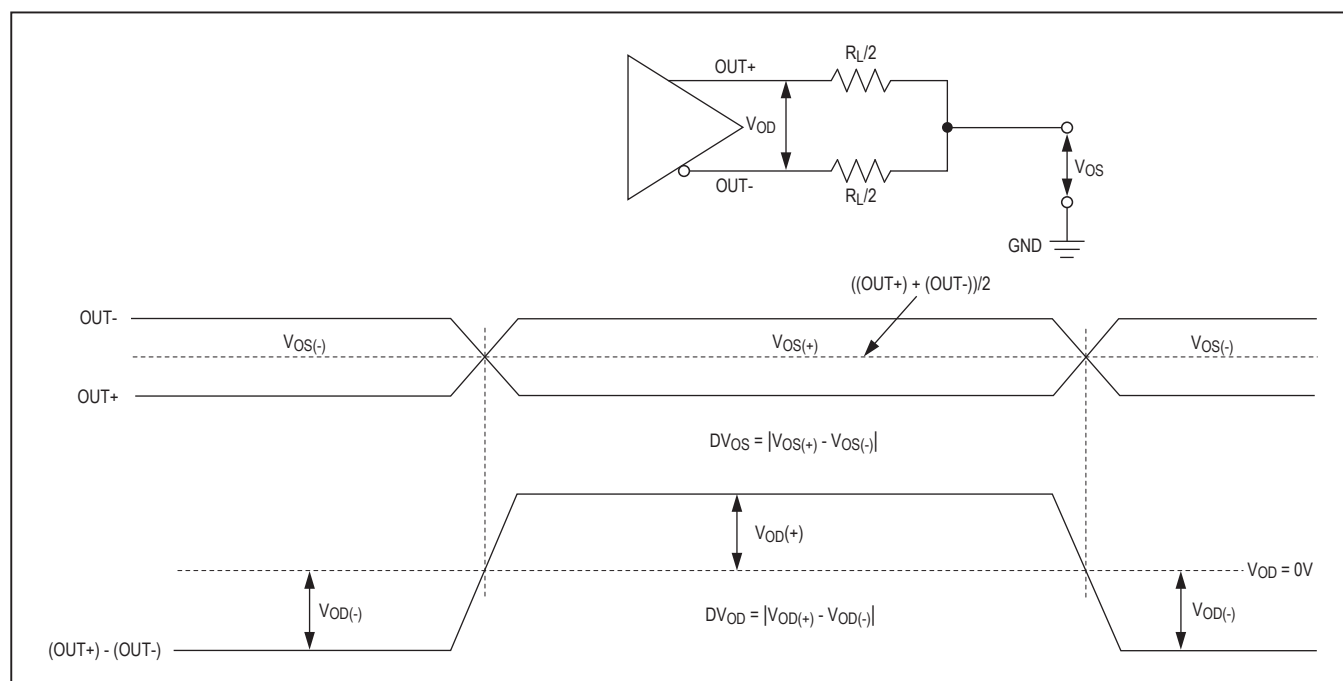
Figure 1. Serial-Output Parameters
