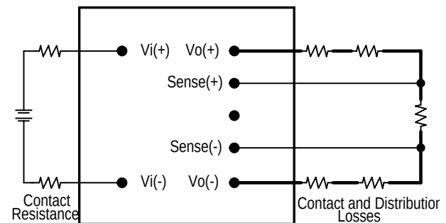
Figure 16: Effective circuit configuration for remote sense operation
