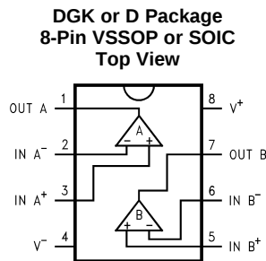
Pin Functions – LMV342-N
