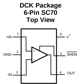
Pin Functions – LMV341-N
