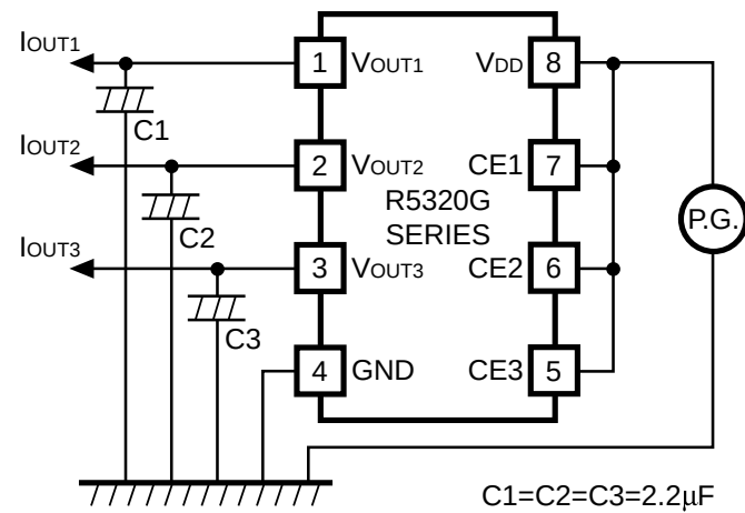
Test Circuit for Line Transient Response
