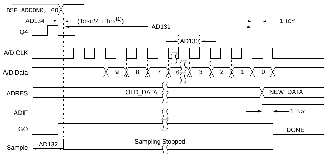
FIGURE 16-11: PIC12F615/617/HV615 A/D CONVERSION TIMING (SLEEP MODE)
