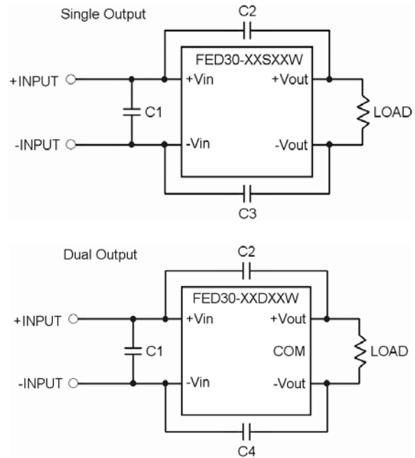
Recommended Filter for EN55022 Class A Compliance
