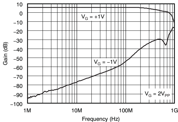
Figure 16. Fully-Attenuated Response
