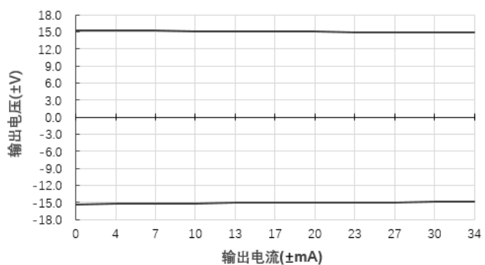
输出电压Vs输出电流(Vin=12V)@A1215S-1WR3
