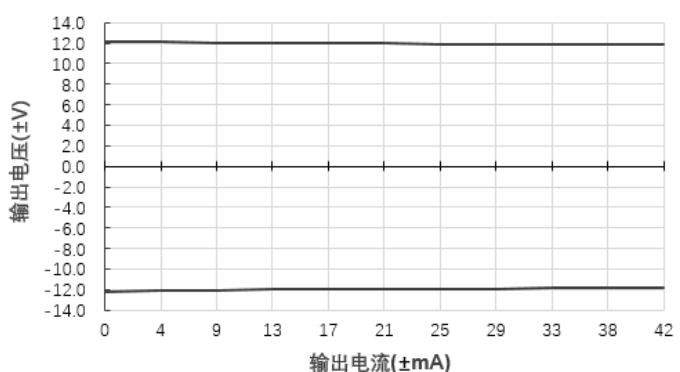
输出电压Vs输出电流(Vin=24V)@A2412S-1WR3
