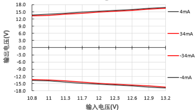
输出电压Vs输入电压@A1215S-1WR3
