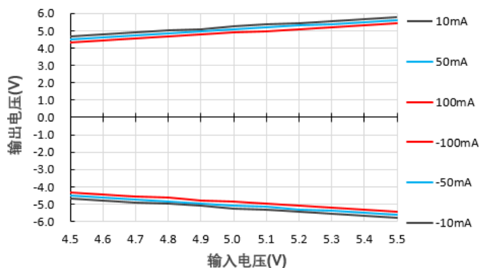
输出电压Vs输入电压@A0505S-1WR3
