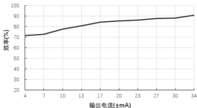
效率Vs输出电流(Vin=24V)@A2415S-1WR3
