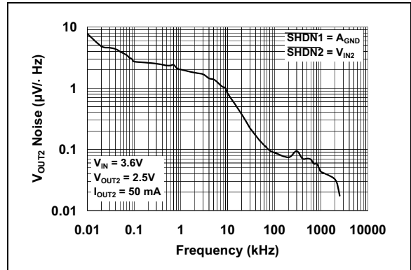
FIGURE 2-34: V_{OUT2} Noise vs. Frequency.
