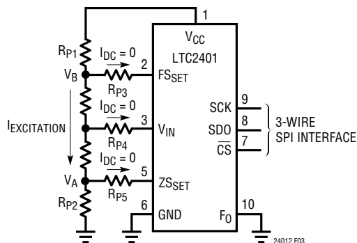
Figure 3. Half-Bridge Digitizer with Zero-Scale and Full-Scale Sense
