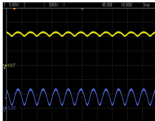
Figure 10. Output Voltage & Current at 230V AC
