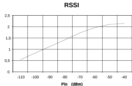
Figure 9. RSSI Voltage
