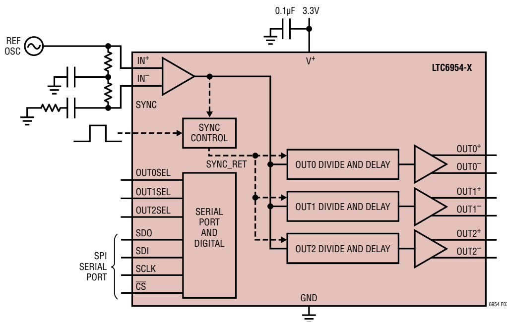
Figure 7. SYNC_RET Propagation
