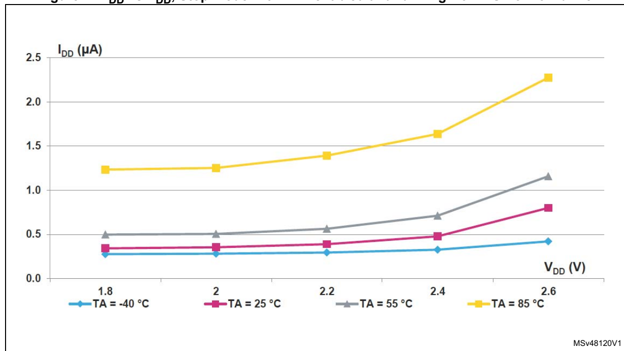
Figure 11. I_{DD} vs V_{DD} , Stop mode with RTC enabled and running from LSE on low drive
