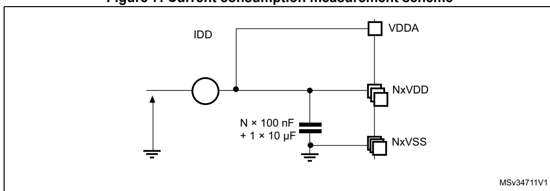
Figure 7. Current consumption measurement scheme
