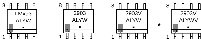
SOIC-8 CASE 751
