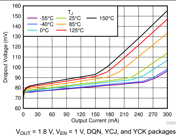
Figure 6-29. Dropout Voltage vs I_{OUT}
