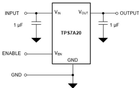
Simplified Schematic
