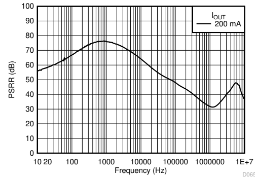
Figure 8-6. PSRR
