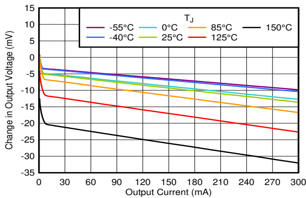
V_{IN} = 2.8 \text{ V} , V_{EN} = 1 \text{ V} , DBV package Figure 6-7. Load Regulation vs I_{OUT}
