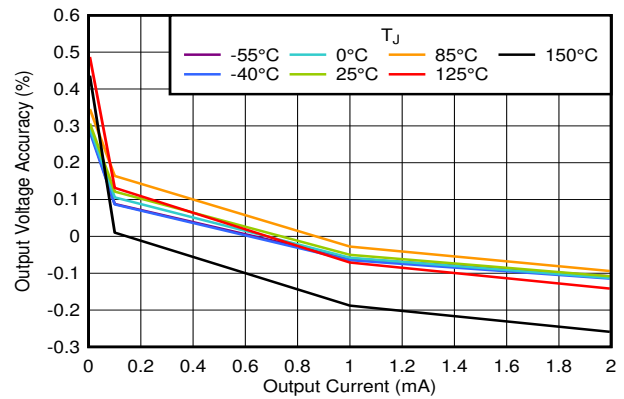
Figure 6-14. Output Voltage Accuracy vs I_{OUT}
