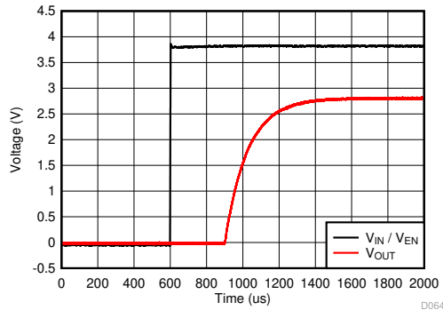
Figure 8-5. Start-Up
