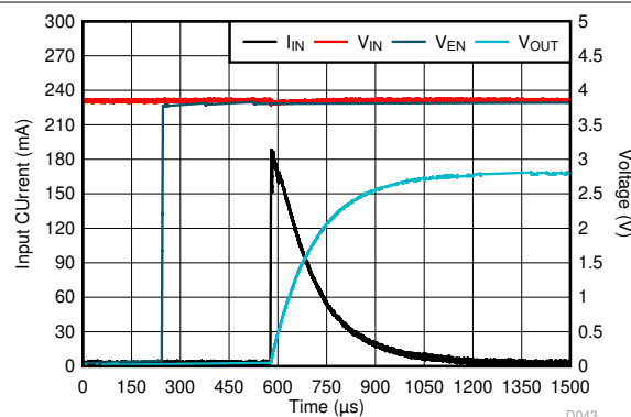
Figure 6-82. Start-Up
