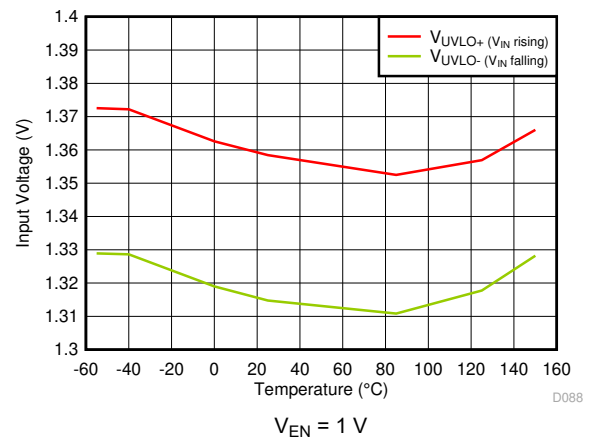
Figure 6-46. UVLO Threshold vs Temperature
