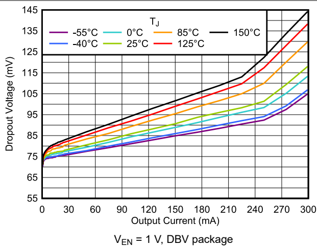
Figure 6-27. Dropout Voltage vs I_{OUT}
