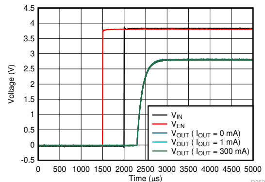
Figure 6-76. Start-Up
