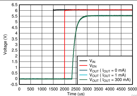
Figure 6-80. Start-Up
