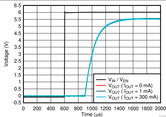
Figure 6-80. Start-Up
