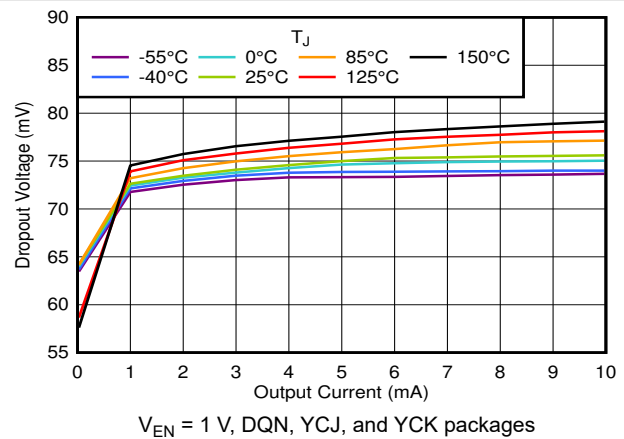
Figure 6-26. Dropout Voltage vs I_{OUT}
