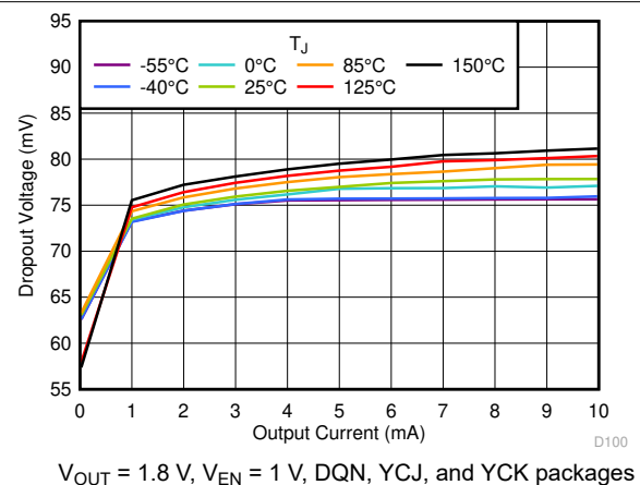
Figure 6-30. Dropout Voltage vs I_{OUT}
