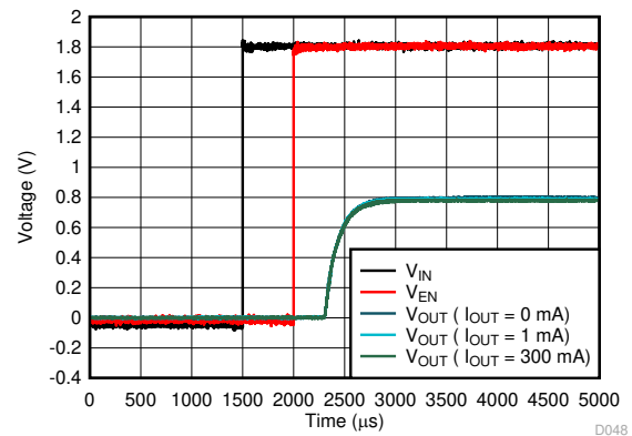
Figure 6-74. Start-Up
