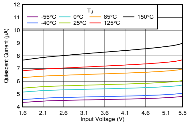
Figure 6-37. I_{GND} vs V_{IN} in the Dropout Region
