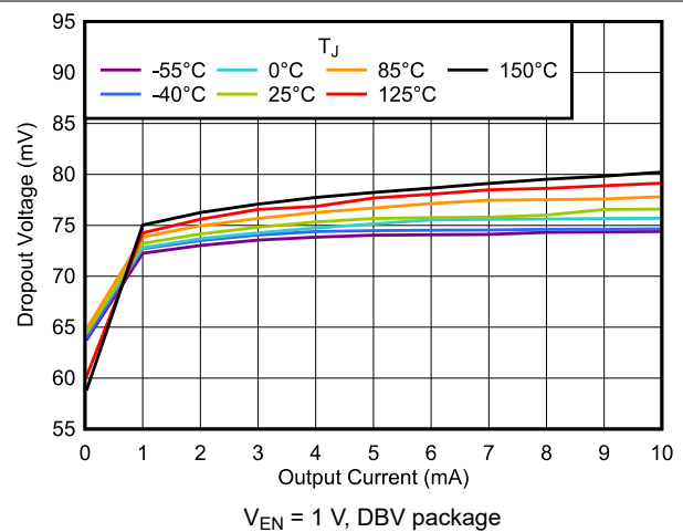
Figure 6-28. Dropout Voltage vs I_{OUT}
