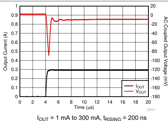
Figure 6-53. Load Transient
