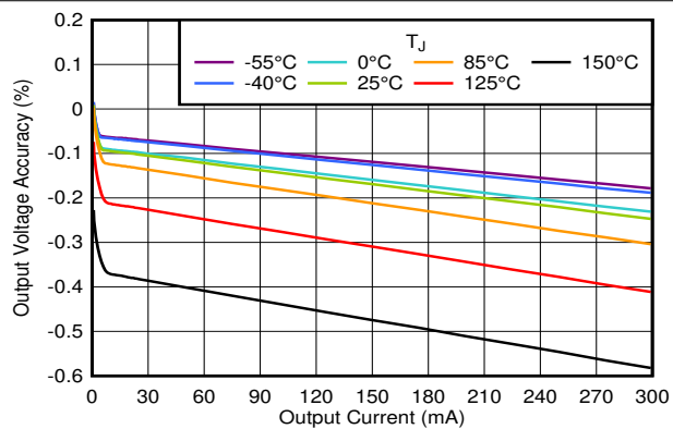
Figure 6-15. Output Voltage Accuracy vs I_{OUT}
