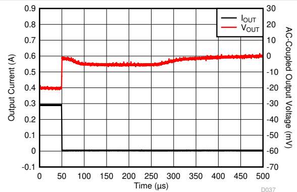
Figure 6-56. Load Transient
