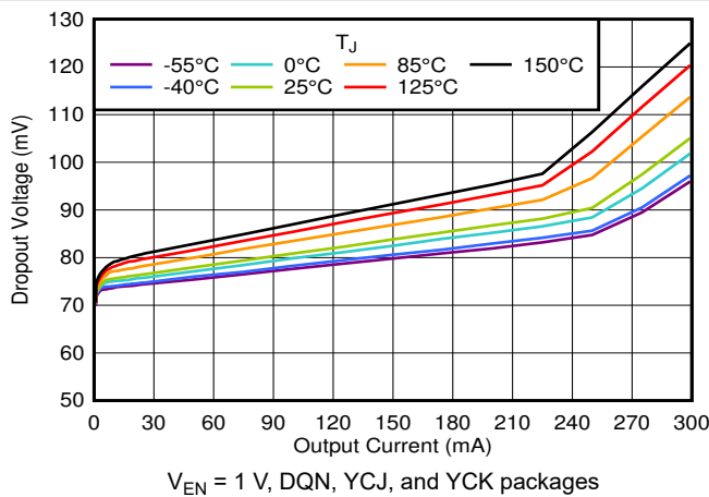
Figure 6-25. Dropout Voltage vs I_{OUT}
