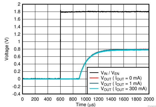
Figure 6-74. Start-Up
