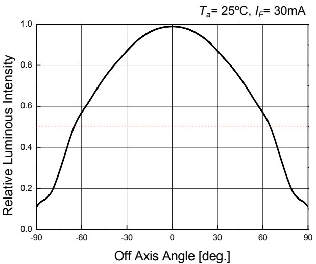
Directivity
