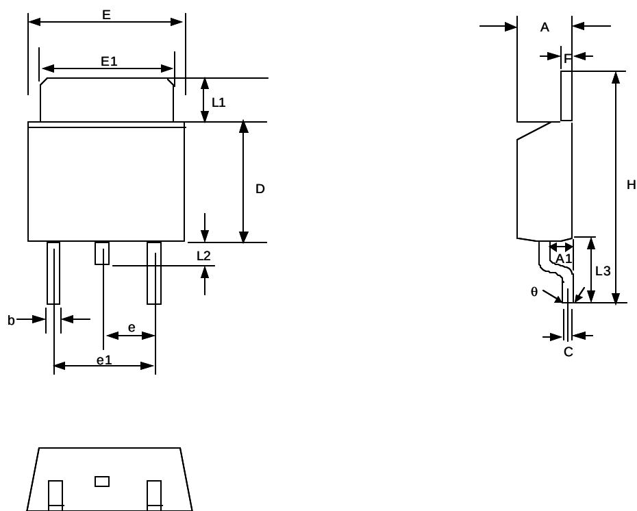
TO-252 (GT4) Package
