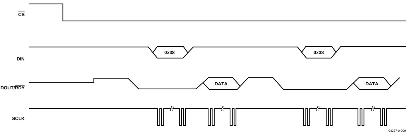
Figure 14. Continuous Conversion
