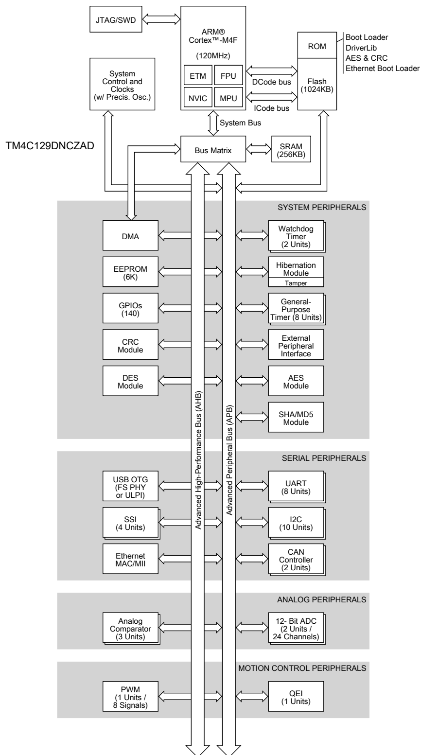
Figure 1-1. Tiva™ TM4C129DNCZAD Microcontroller High-Level Block Diagram
