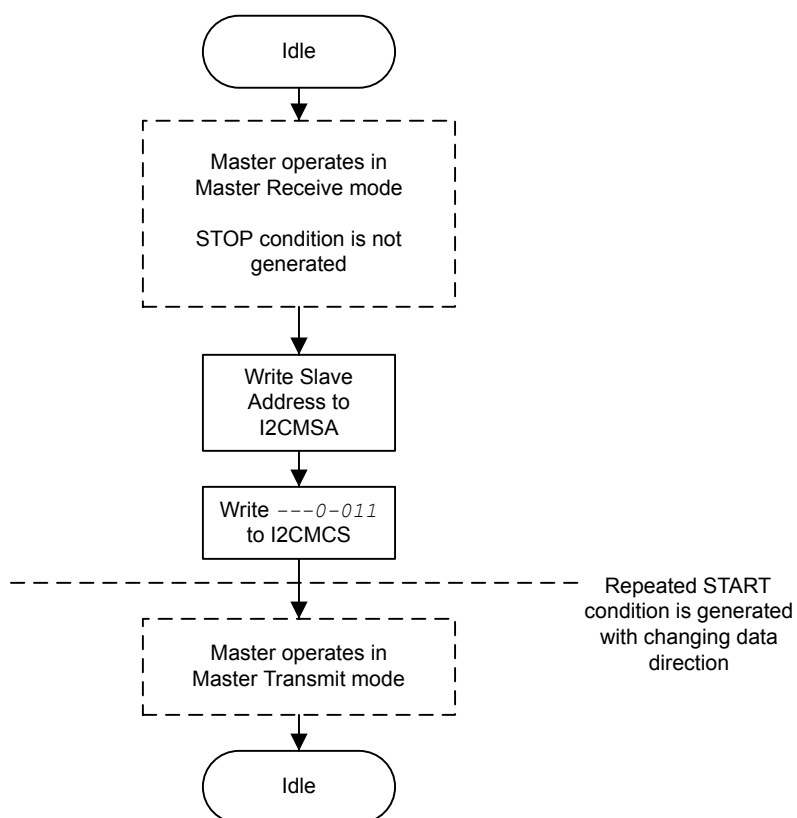
Figure 21-13. Master TRANSMIT with Repeated START after Master RECEIVE
