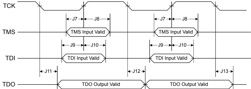
Figure 30-3. JTAG Test Access Port (TAP) Timing
