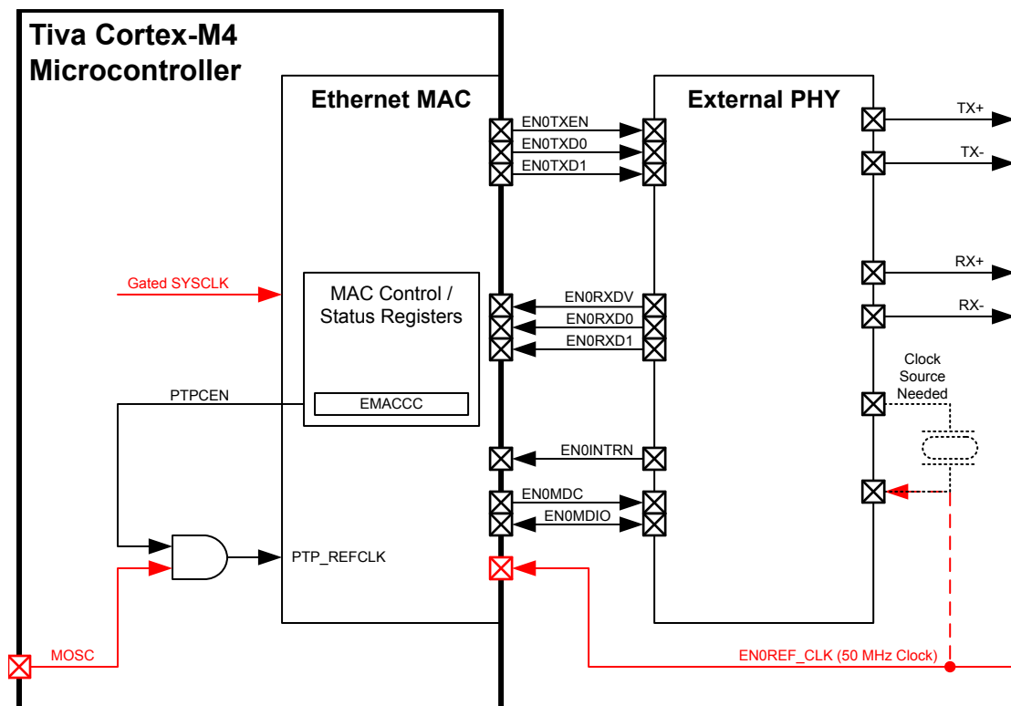
Figure 23-3. RMII Clock Structure
