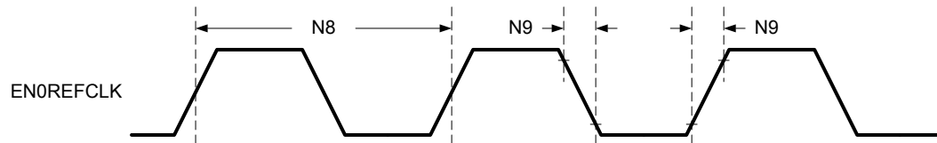
Figure 30-36. EN0RREF_CLK 50-MHz Oscillator Characteristics
