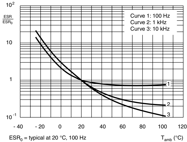
Fig.4 Typical multiplier of ESR as a function of ambient temperature at different frequencies
