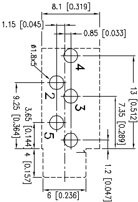
HOLE LAYOUT (TOP VIEW)
